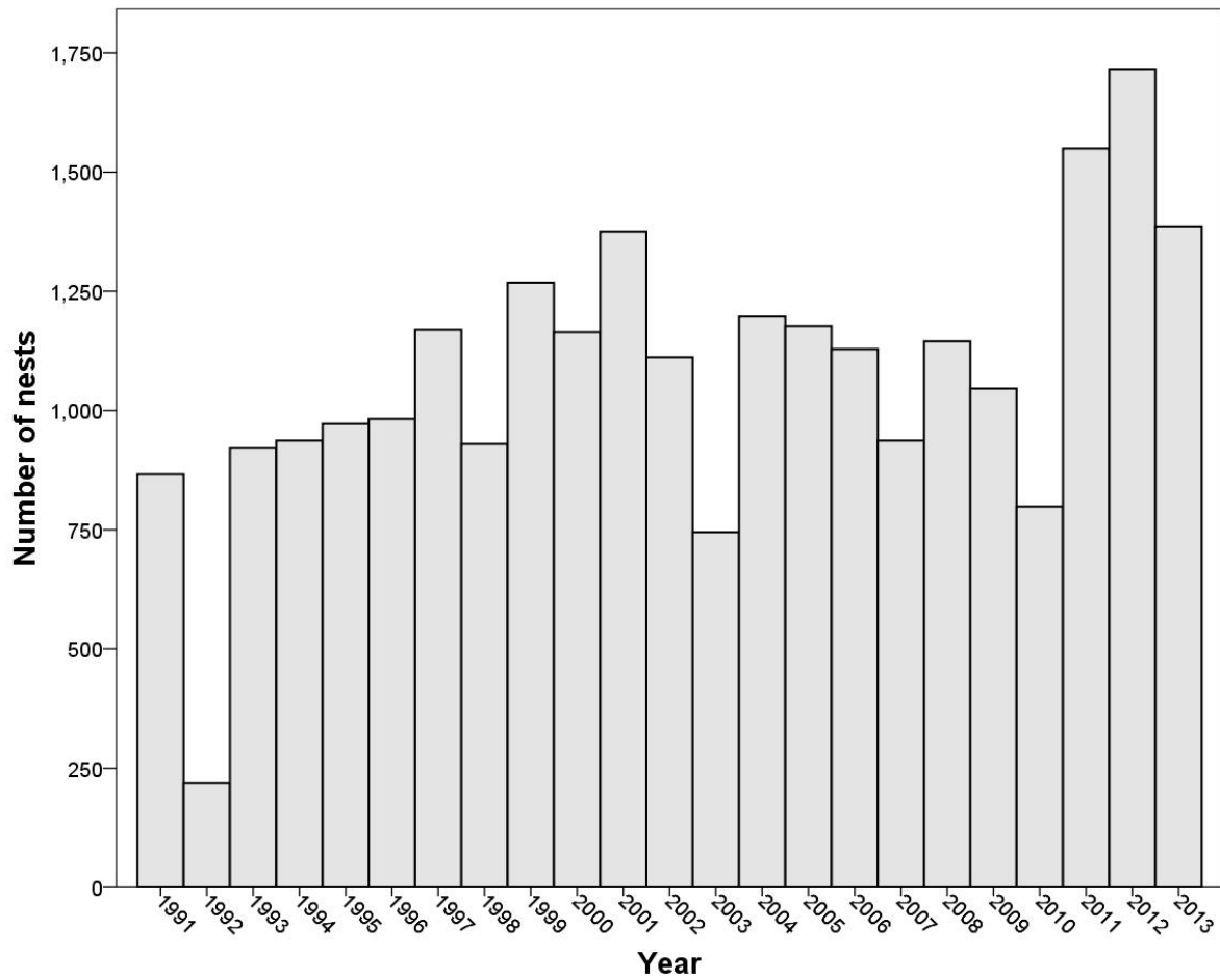
Fig A1. Number of breeding pairs of blue-footed boobies recorded every year in a fixed study area measuring 26 889 m 2 on Isla Isabel over the 23 years from 1991 to 2013. This pattern is consistent with interannual variation in population size estimated by the mark-recapture data.
